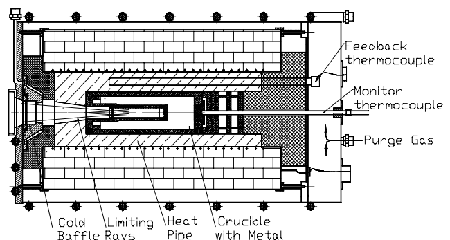
Figure 1. Fixed-point blackbody schematic for Al and Ag.
