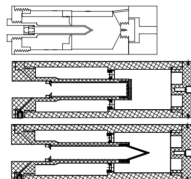
Figure 2. Three fixed-point cavities evaluated in this study.
